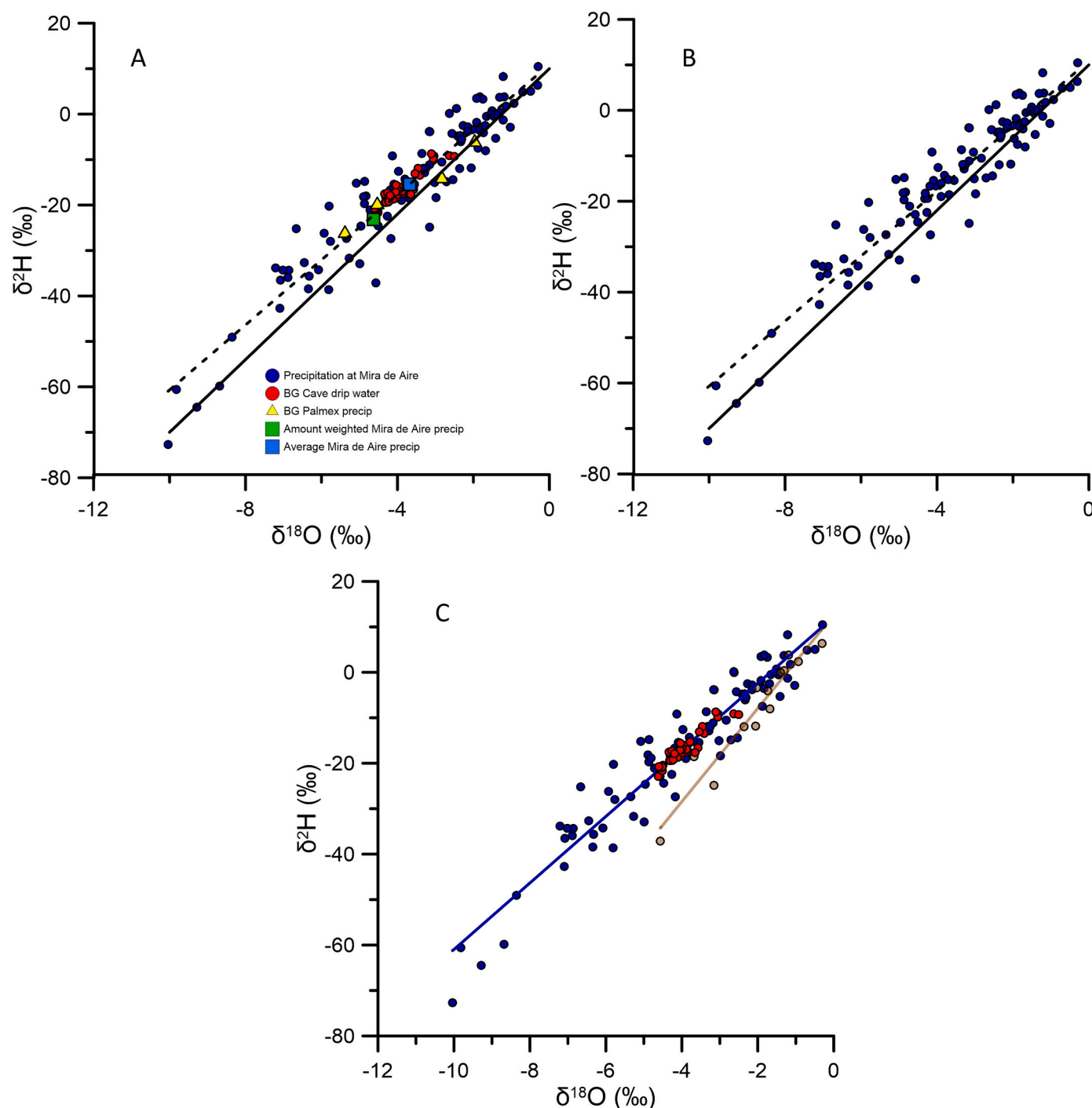
Fig. 6. A. Mirade Aire precipitation (blue circles), BG cave drip water (red circles), BG bulk precipitation (yellow triangles), Mira de Aire amount-weighted average precipitation (green square), Mira de Aire average precipitation (light blue square), Mira de Aire LMWL (dashed), and GMWL (solid black). B. Rainfall data from Mira de Aire (~5 km from BG) with LMWL (dashed) and GMWL (solid) shown. C. Wet season LMWL (October–April, blue) and dry season LMWL (May–September, brown) with BG cave drip water (red). (For interpretation of the references to colour in this figure legend, the reader is referred to the web version of this article.)
